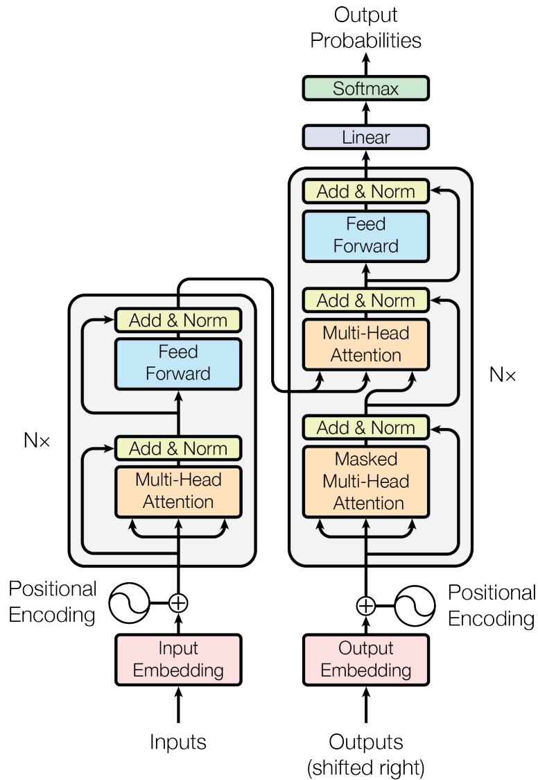
Figure 3.1: Transformer Architecture
